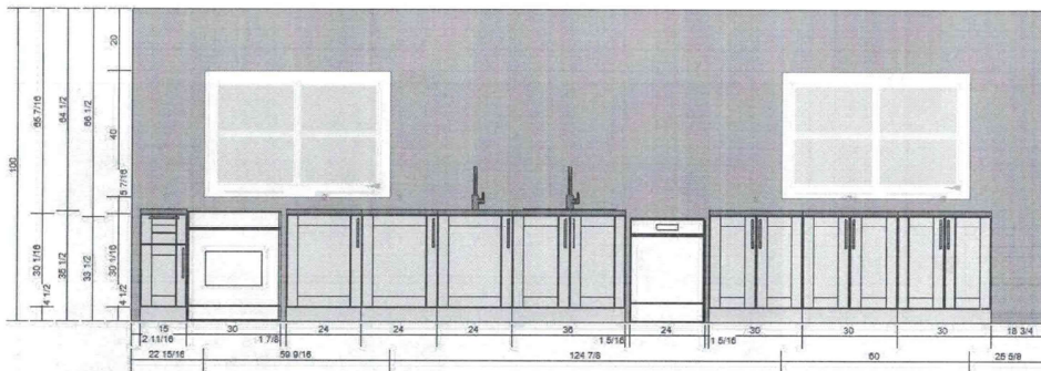
Figure 2 Cabinets Front View, North Wall
